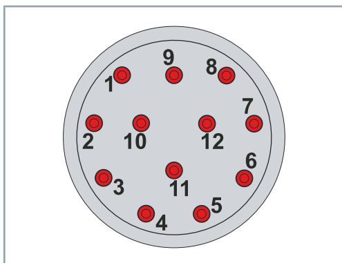
Pin assignment of 12-pin Speedtec connector
