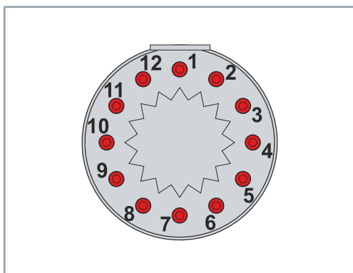
Pin assignment of yTec 12-pin connector
